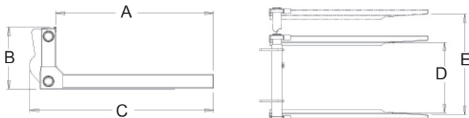
48" bale squeeze
